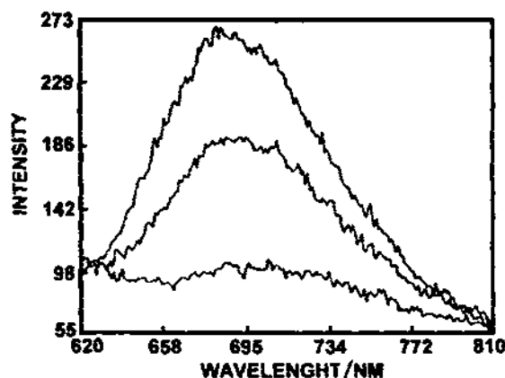
Fig. 9. Uncorrected emission spectra of ^*Cu(dmp)_2^+ in 4:1 ethanol + methanol. In order of decreasing emission intensity, the sample temperature was 90 K, 100 K and 110 K. (Reproduced with permission from Ref. [35].)
