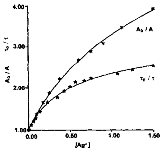
Fig. 8. Luminescence intensity (*) and lifetime (★) Stern–Volmer quenching plots for the \text{Ru}(\text{bpy})_3^{2+} – \text{Ag}^+ system at an ionic strength of 3 M. (Reproduced with permission from Ref. [29].)
