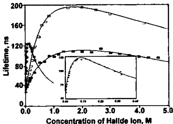
Fig. 13. Dependence of the luminescence lifetime on the concentration of halide ion in aqueous solutions of \text{Cu}(\text{CN})_2^- + \text{X}^- at 5 M ionic strength: ■ X = Cl; □ X = Br, ★ X = I. (Reproduced with permission from Ref. [40].)
